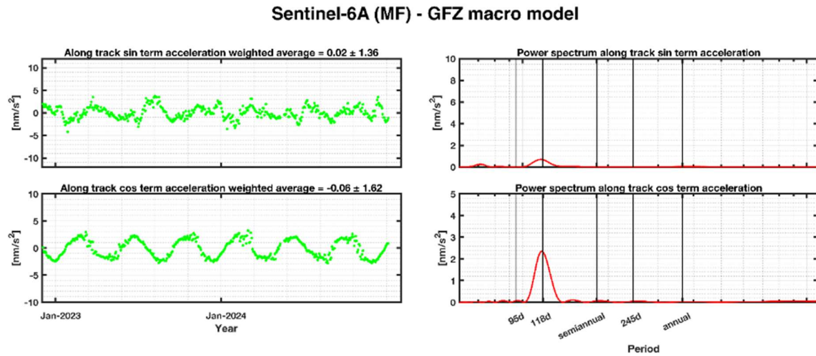
Figure 39. Empirically estimated along-track accelerations (left) and corresponding power spectrum (right) for the GFZ macro model.
