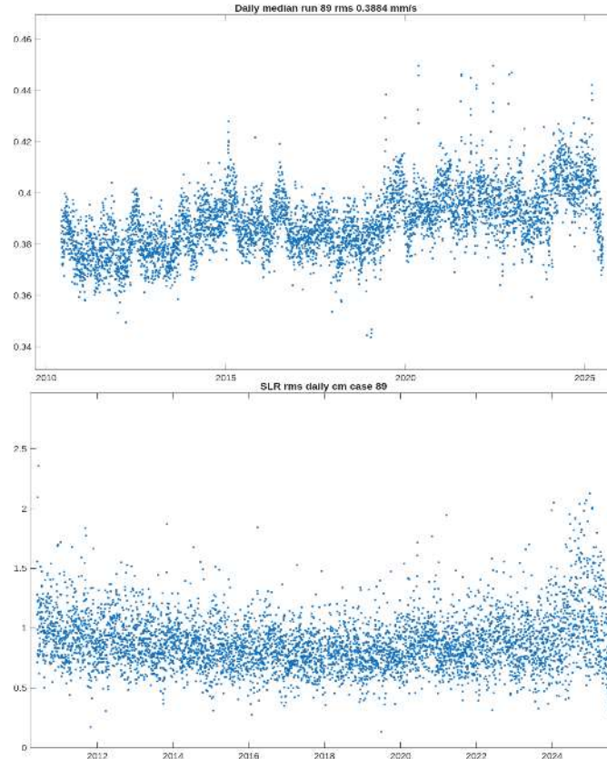
Figure 42. Mean daily tracking residuals for DORIS (top) and SLR (bottom).
