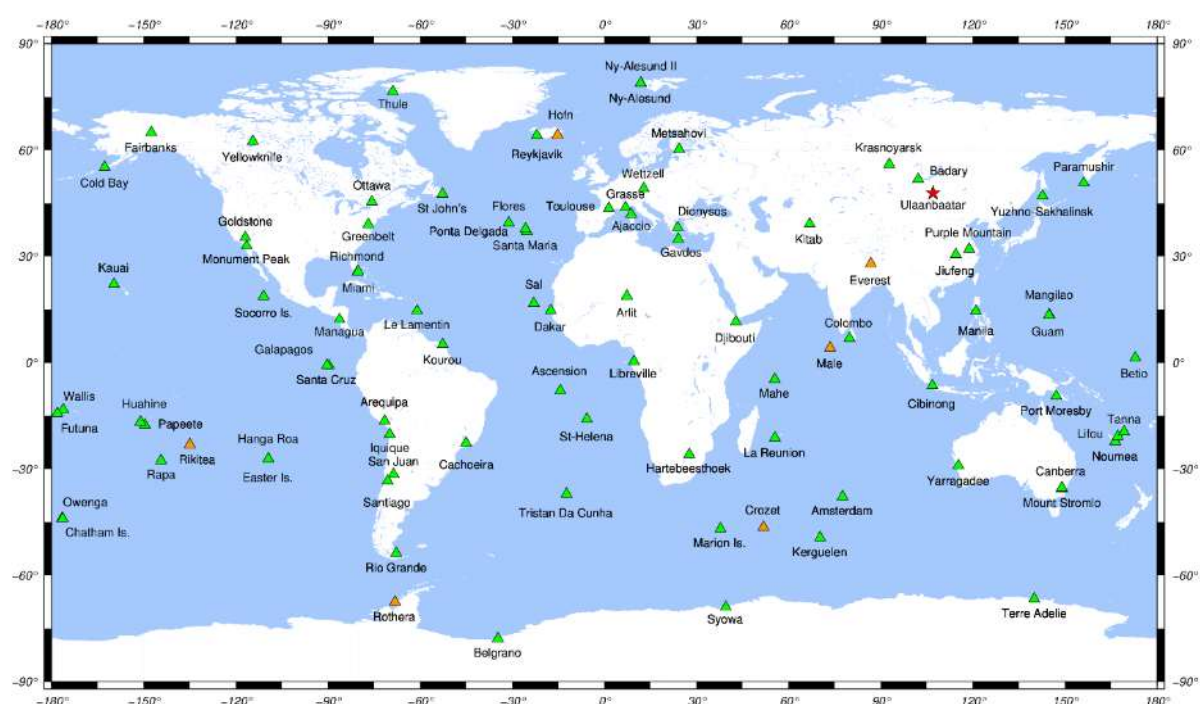
Figure 18. ITRF2020-u2024 DORIS beacon ground network (in green: sites with no new beacon since ITRF2020-u2023; in orange: sites with new beacon since ITRF2020-u2023; in red: new site since ITRF2020-u2023).
