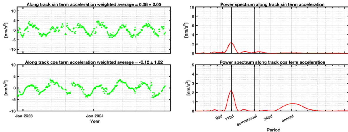
Figure 40. Empirically estimated along-track accelerations (left) and corresponding power spectrum (right) for the Conrad macro model
