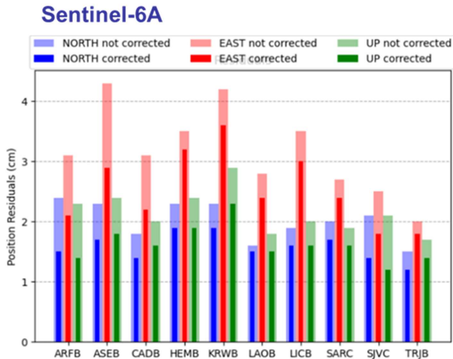
Figure 24. Standard deviation of NEU components for SAA stations (with / without GPS clock corrections).
