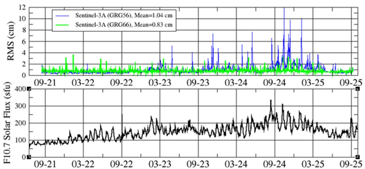
Figure 28. RMS radial orbit differences vs solar flux 10.7 (Sentinel 3A).
