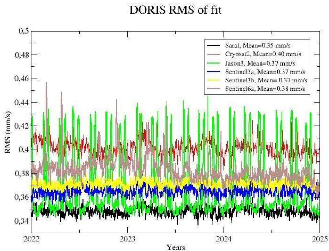
Figure 29. DORIS RMS of fit for Saral, Cryosat2, Jason3, Sentinel3a, Sentinel3b and Sentinel6a satellites for 2022.0-2025.0.
